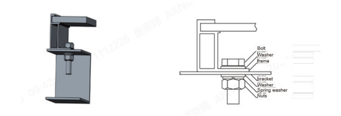
Module Mounting Holes
