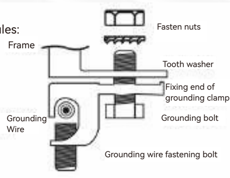
Figure 10 Bolt Grounding Method of PV Module
