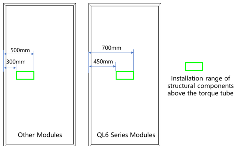
Figure 12. Diagram of horizontal installation distance for tracker components above the torque tube.
