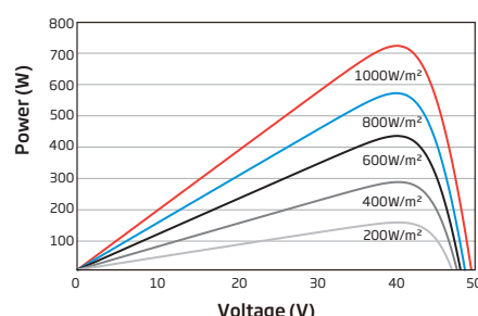
P-V CURVES OF PV MODULE (730W)
