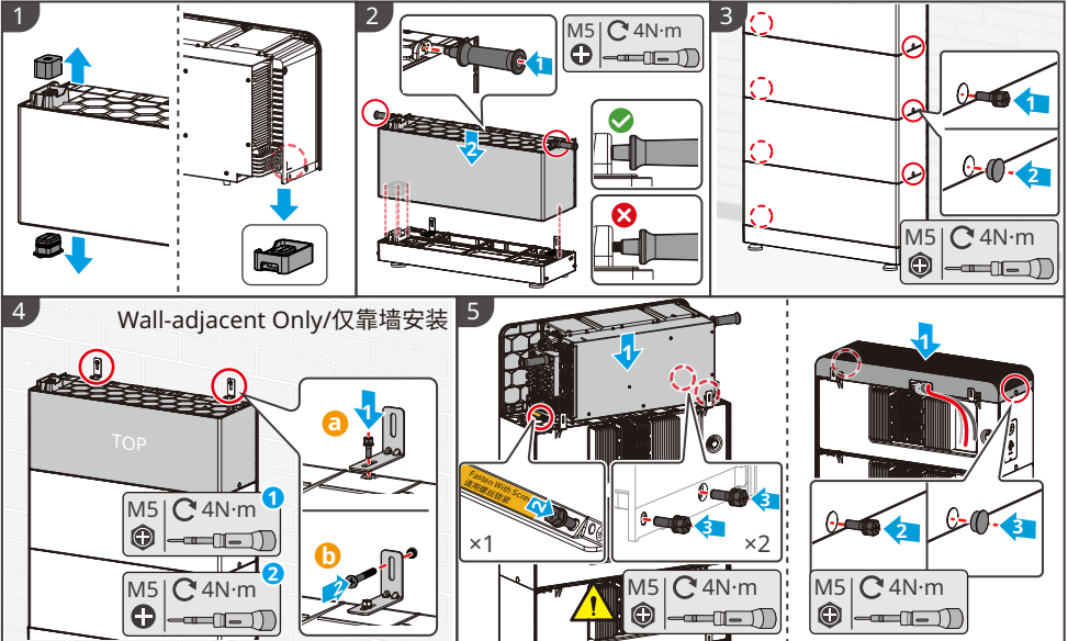
Installation of battery , inverter & battery protective cover. /安装电池、逆变器和电池防护罩
