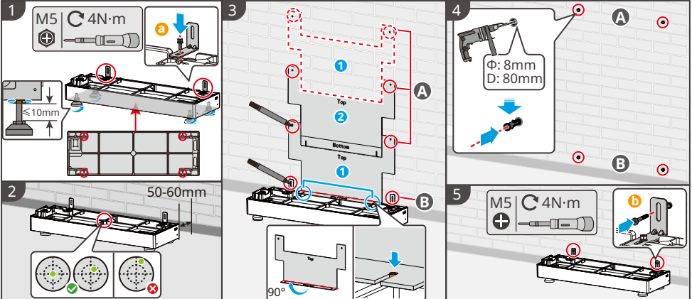
Free-standing Installation/离墙安装
