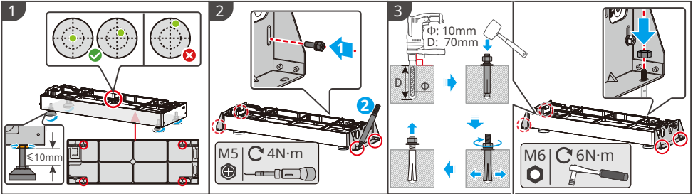
Installation of battery , inverter & battery protective cover. /安装电池、逆变器和电池防护罩
