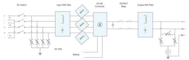
SUN2000-8/10K-LCO
